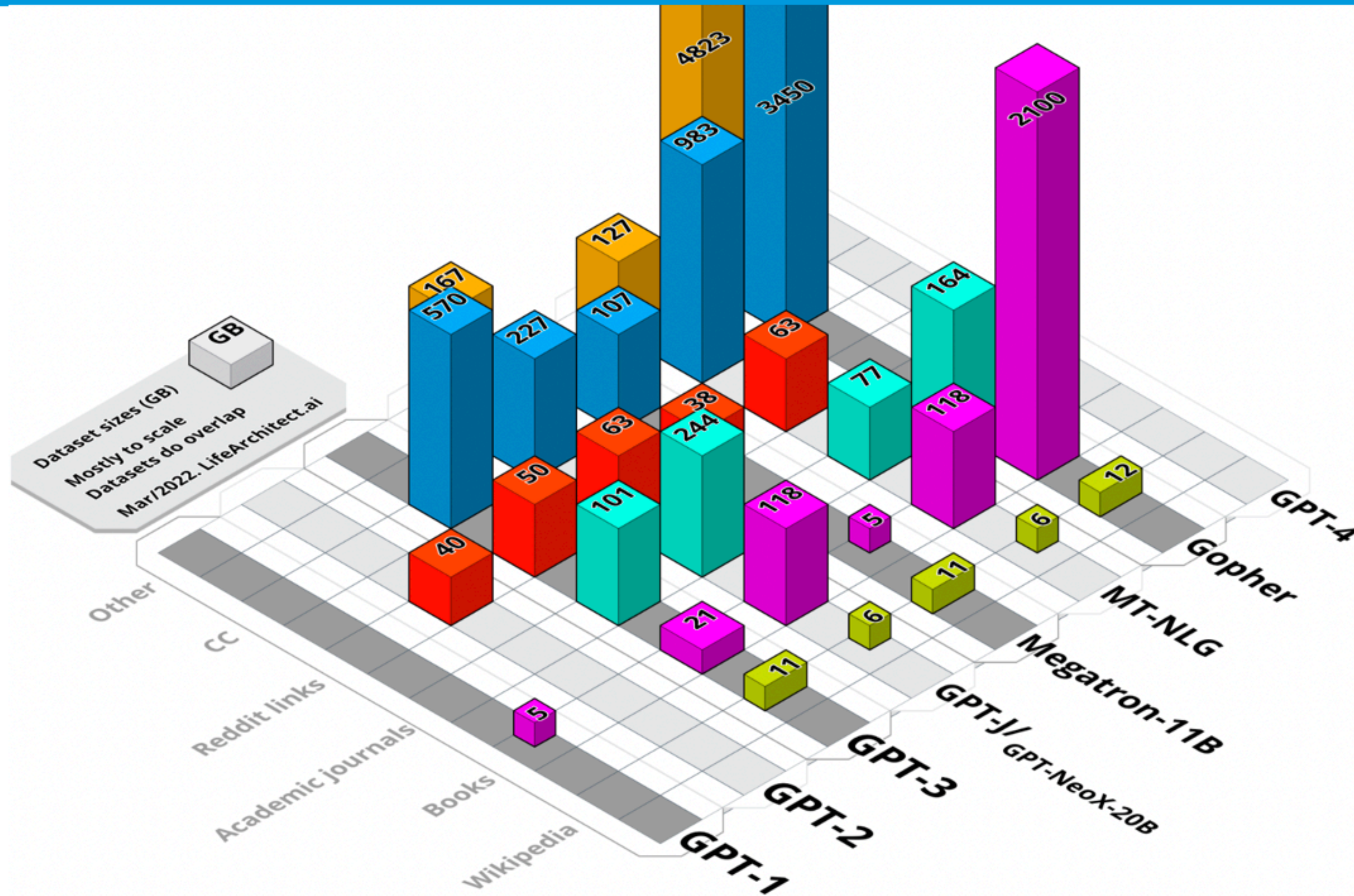
Common Crawl
